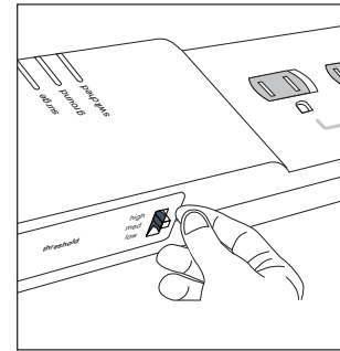
Step 4 Adjust switching threshold, typically "high" for TV applications
